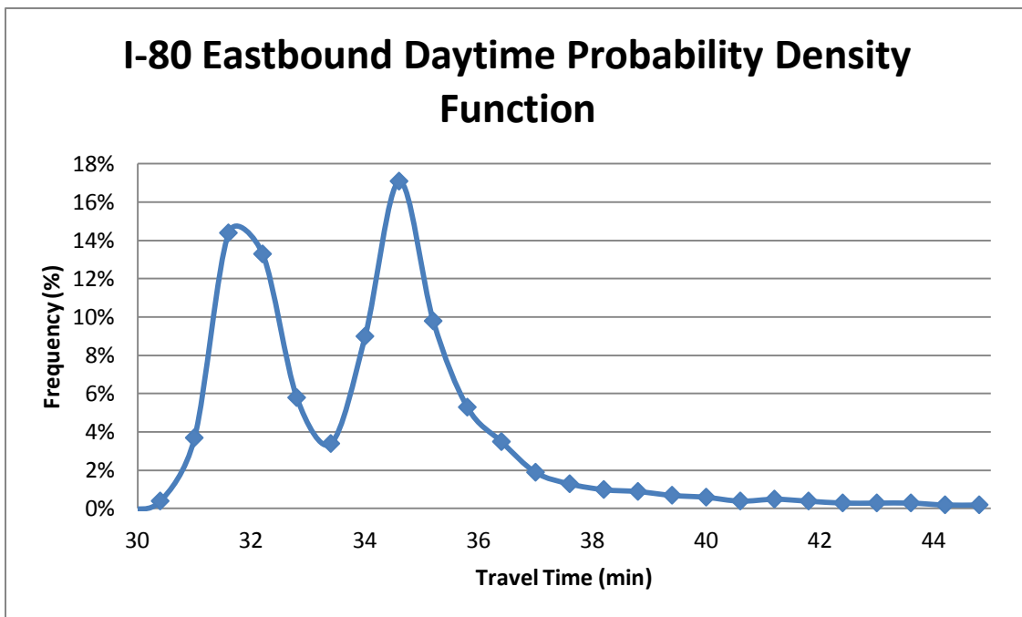
Figure 20: Graph. Eastbound Travel Time Frequency, Daytime
