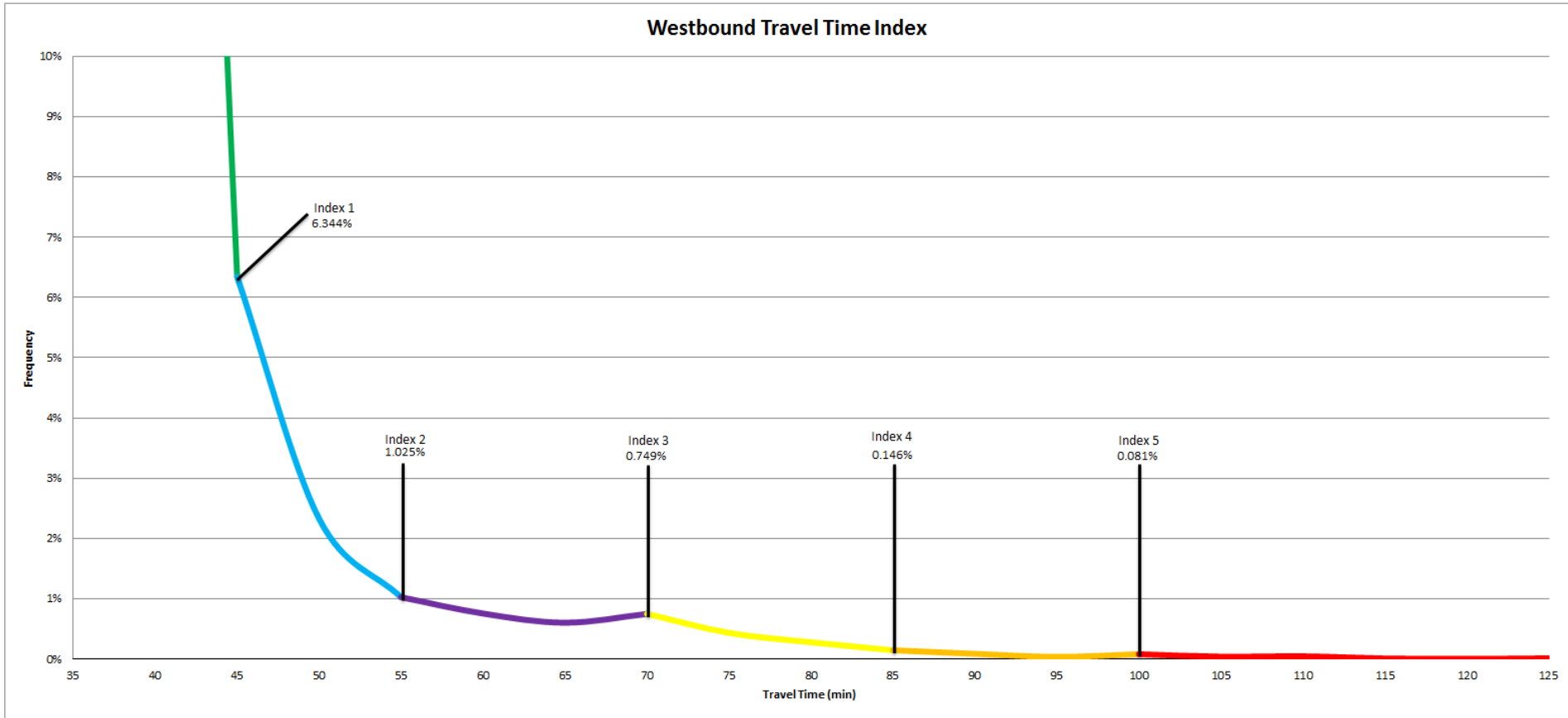
Figure 28: Graph. Westbound Travel Time Index for I-80 between Cheyenne and Laramie
