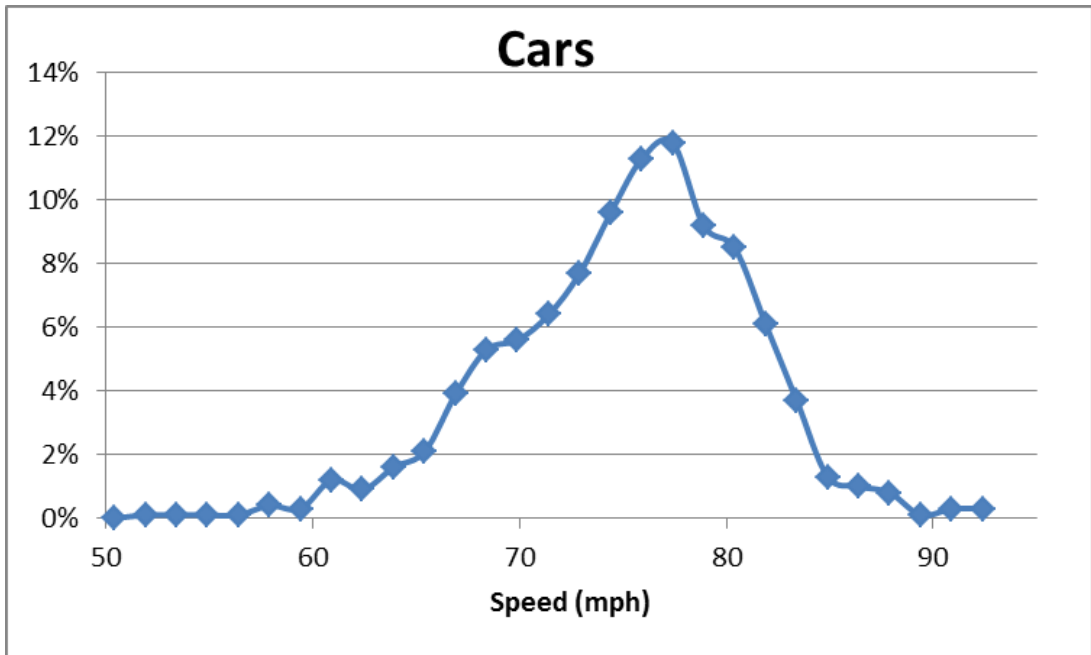
Figure 22: Graph. Elk Mountain Car Speed Frequency
