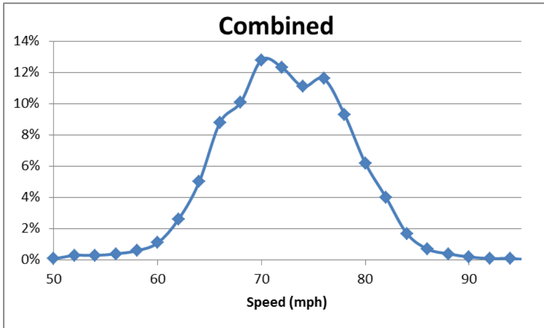
Figure 24: Graph. Elk Mountain Combined Speed Frequency
