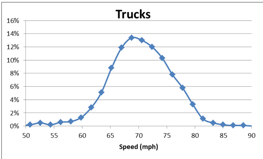
Figure 23: Graph. Elk Mountain Truck Speed Frequency
