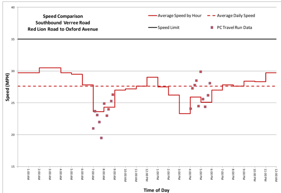
Figure 4: Graph. Bluetooth Sensors vs. Test Car Run Method (6)
