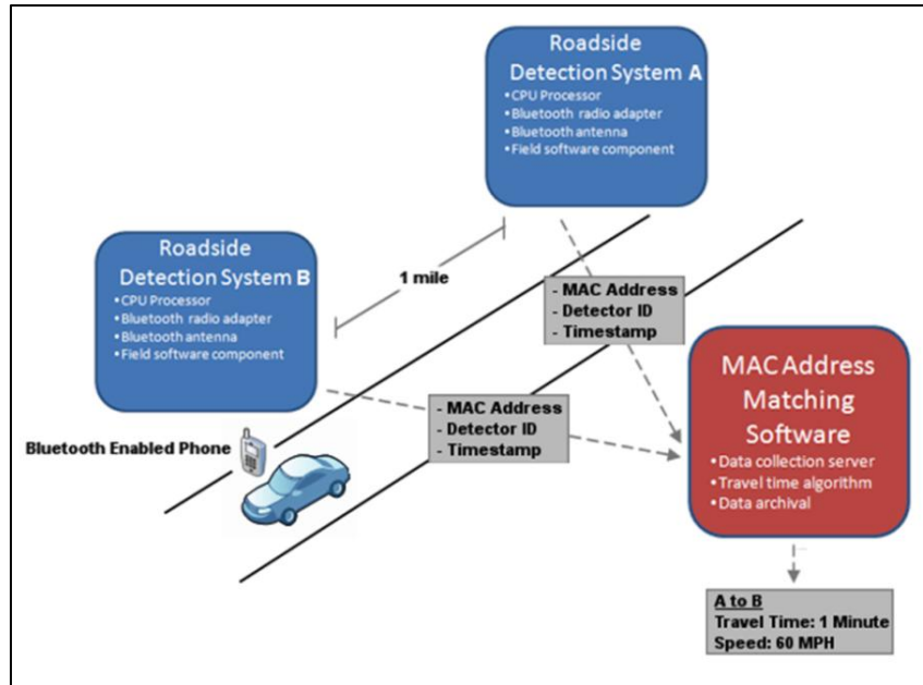
Figure 1: Diagram. MAC Address Matching Method (4)
